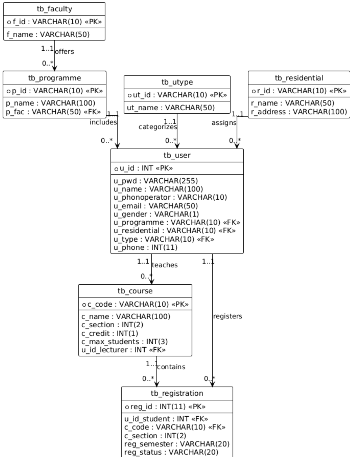
Figure 1.1: Entity Relationship Diagram (ERD)
